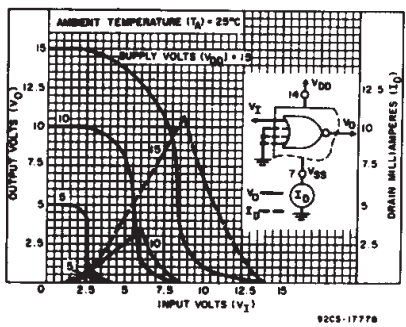
Fig. 3 - Typical current & voltage transfer characteristics.
